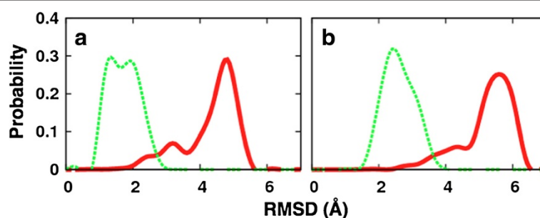
Figure 6 Distributions of the root-mean-square deviation of MD snapshots from the reference X-ray structure (PDB ID: 2V1D). Red: unbound MD ensemble. Green: H3-bound MD ensemble. Either (a) backbone or (b) all-heavy atoms of the residues lining the H3-binding site were considered for least-square fitting and RMSD calculation.
